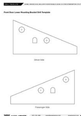
▲ Figure 14. Drill Template Appendix A (appended to the end of this guide)
